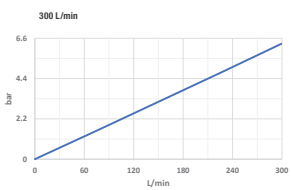
Pressure differential at 30 mm 2 /s
