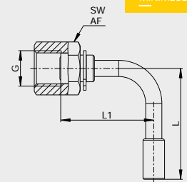
90° pressure gauge fitting as specified in DIN 16288 with O-ring seal
