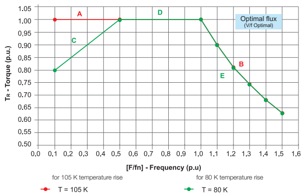
Figure 32 - Derating curves for Optimal Flux condition
