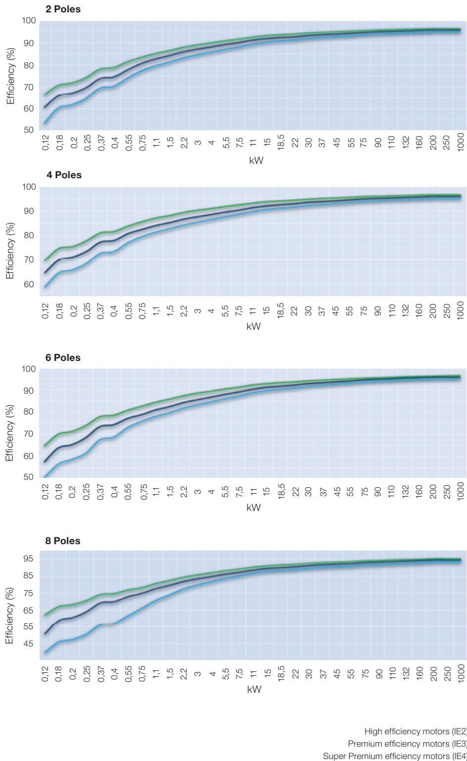
Figure 1 - Efficiency levels according to IEC 60034-30-1 : 2014
