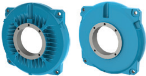
Figure 15 - Drive and non-drive endshields
