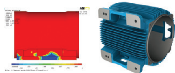
Figure 4 - Solid feet
