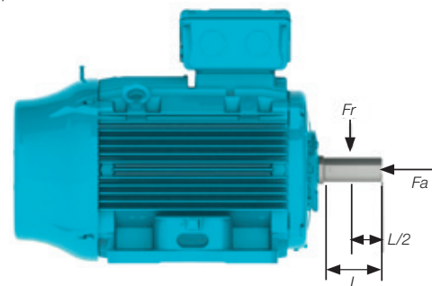
Figure 24 - Radial and axial thrust on motor shaft
