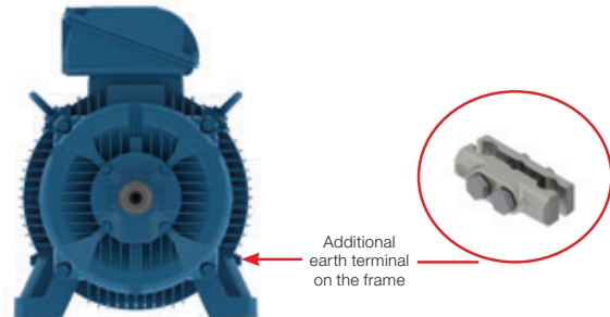
Figure 8 - Additional earth terminal position on the frame.
