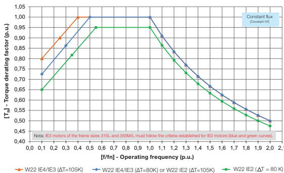
Figure 31 - Derating curves for constant flux condition
