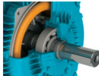
Figure 23 - Ball bearing view
